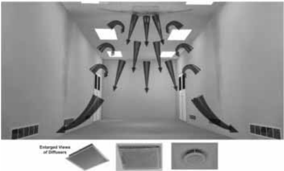
Figure 10 Perforated plate diffuser
